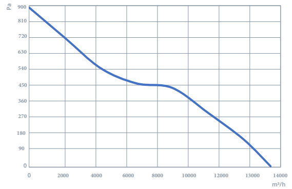
AXI 560-6-45
