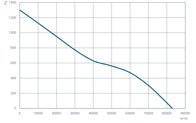
BAXI 1120-8-40
