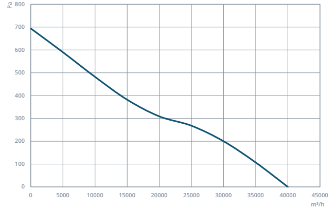
CAXI 900-5-40
