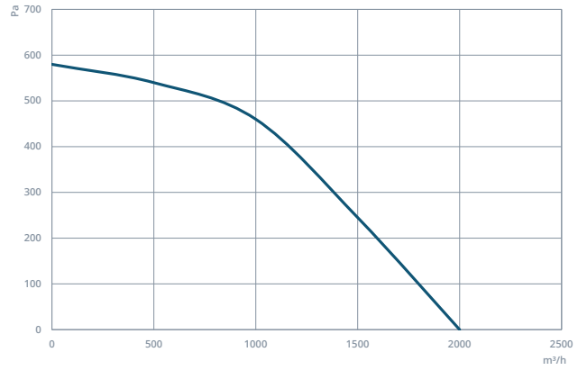
CRAD 280
