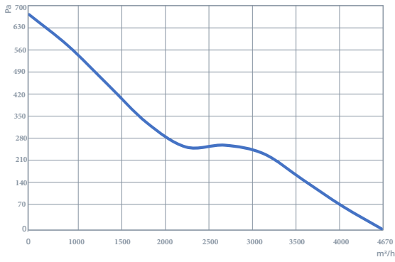
TAXI 315-6-45
