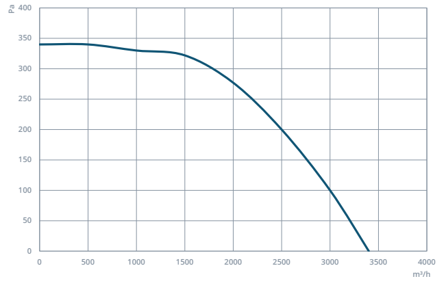
CRAD 400
