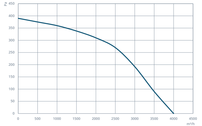
IGK 40
