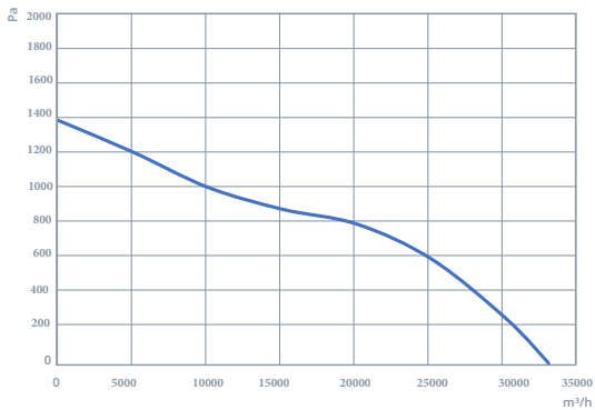
TAXI 630-8-45
