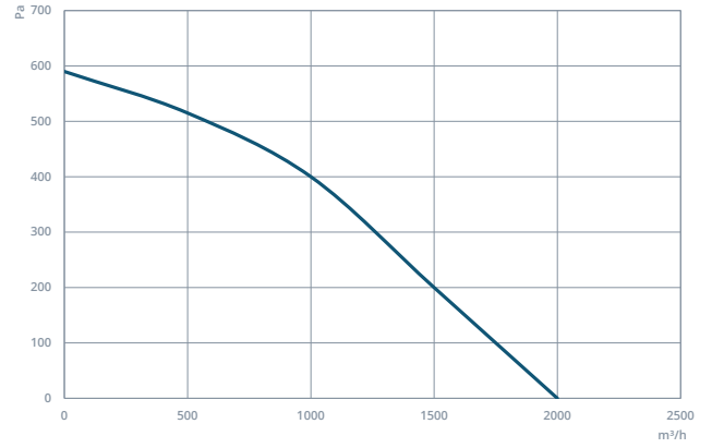
IGK 20
