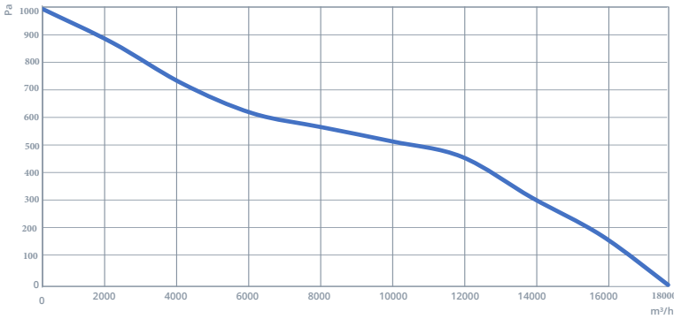
AXI 500-6-45
