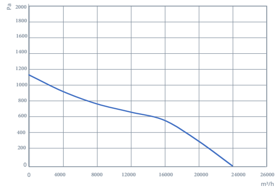
AXI 560-6-45
