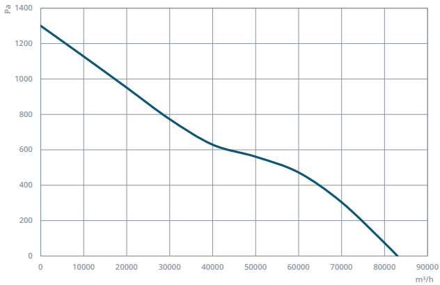
CAXI 1120-8-40
