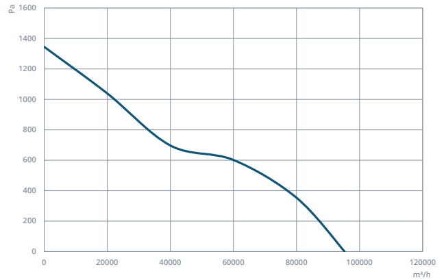
HAXI 1120-8-45
