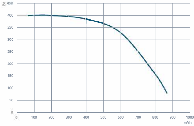
SAF 15
