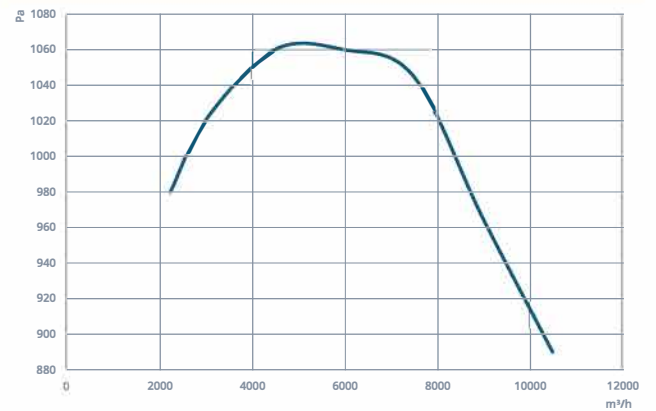
SAF 35
