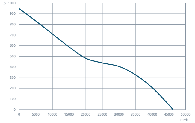
HAXI 900-8-40
