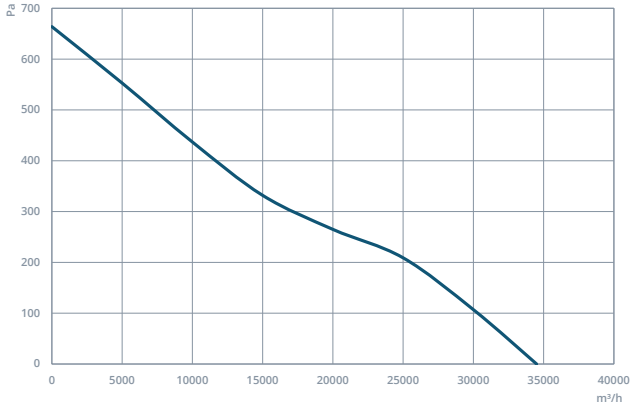
CAXI 900-5-35
