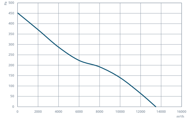
GAXI 630-5-30
