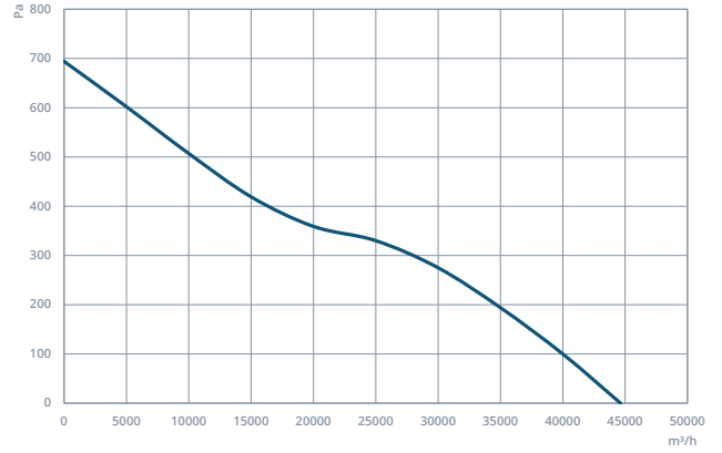
HAXI 900-5-40
