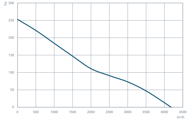
HAXI 450-5-25
