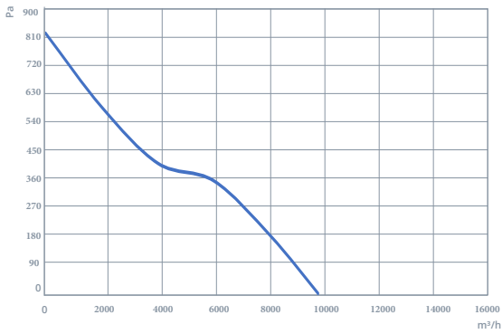
AXI 400-6-45
