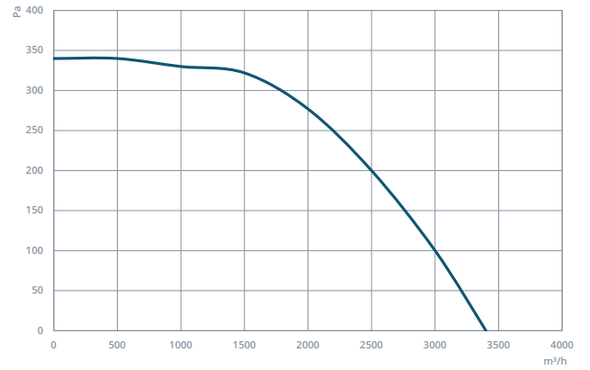
REC 60-35
