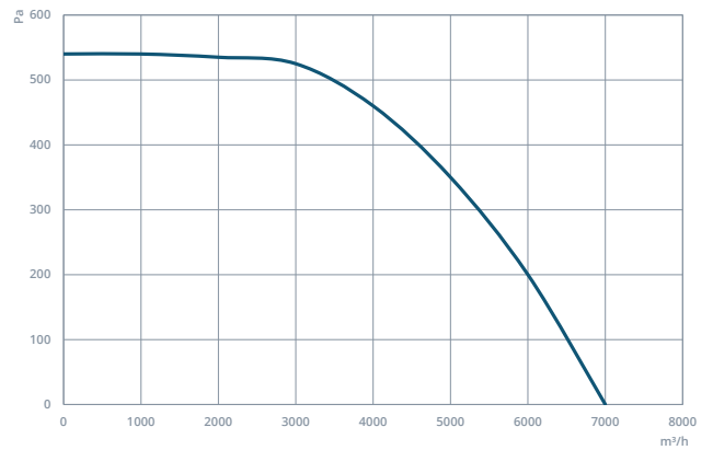
CRAD 500
