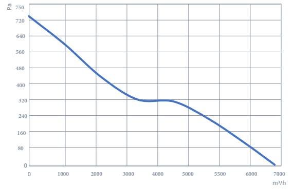
AXI 355-6-45
