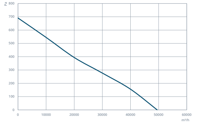
BAXI 1000-5-40
