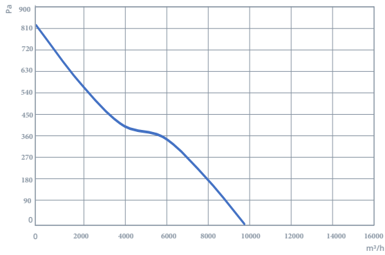
TAXI 400-6-45
