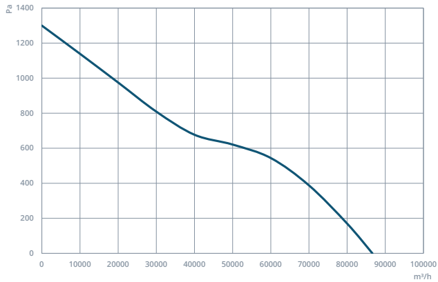
HAXI 1120-8-40
