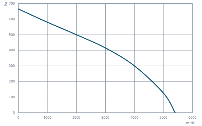
SHU 54
