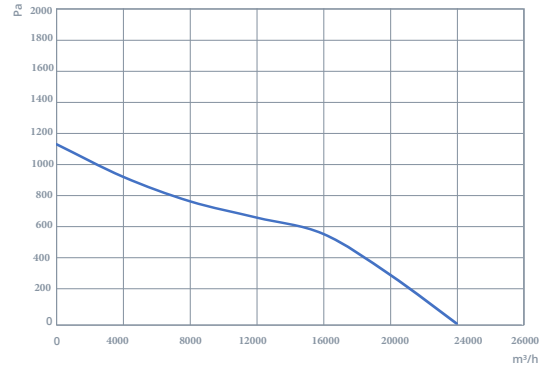
TAXI 560-6-45
