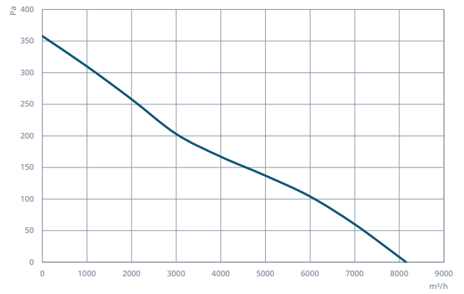
HAXI 560-5-25
