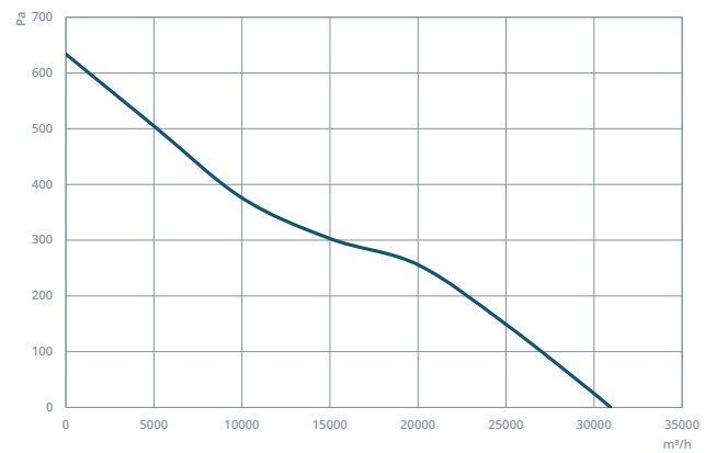
HAXI 800-5-35
