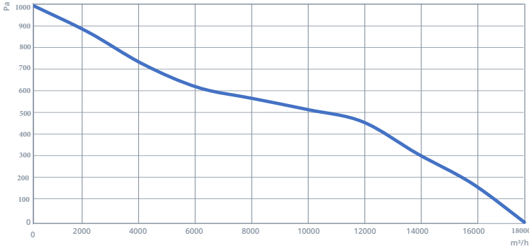
TAXI 500-6-45
